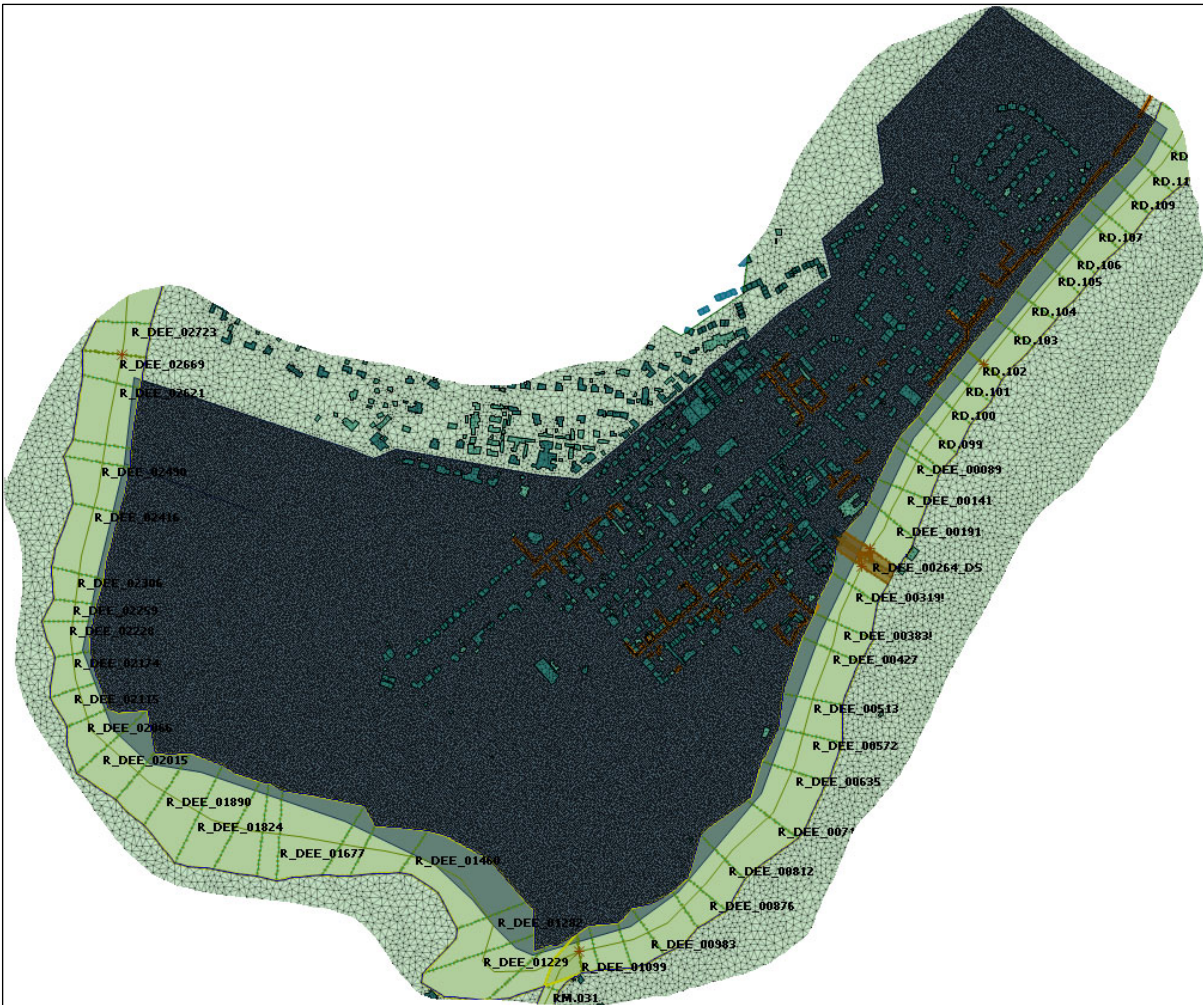
Figure 6.12: Ballater urban mesh zone
