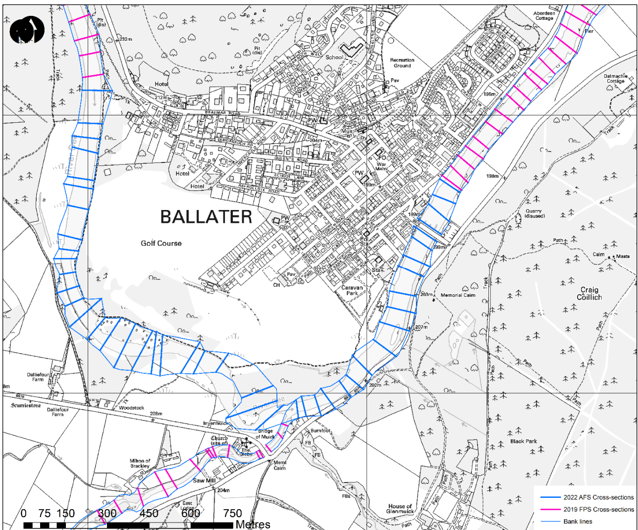
Figure 3.1: Existing and newly surveyed cross-sections for use in the Ballater Additional Flood Study
